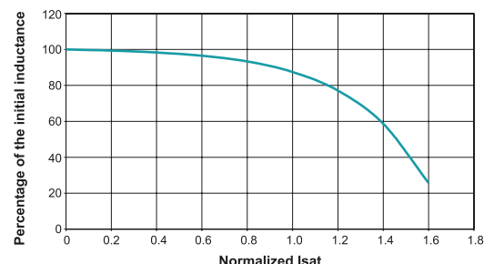
Inductance vs Current Characteristics
