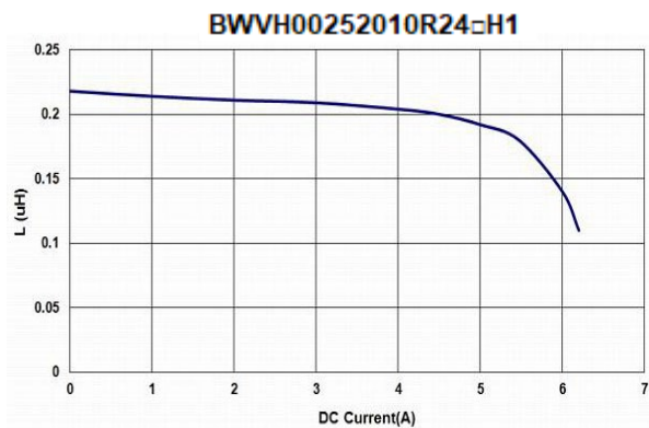
13 Graph: BWVH00252010-H1 Series Graph
