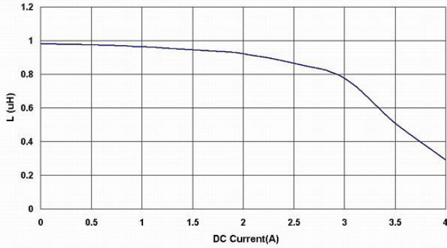
BPSC000505201R5□S0
