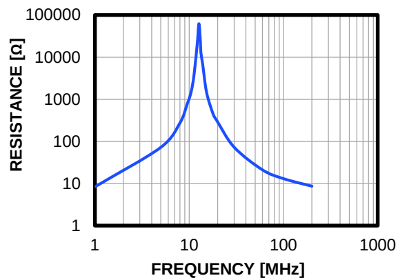
AC Resistance vs. Frequency
