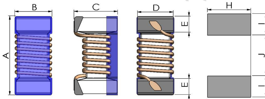
Recommended Land Pattern
