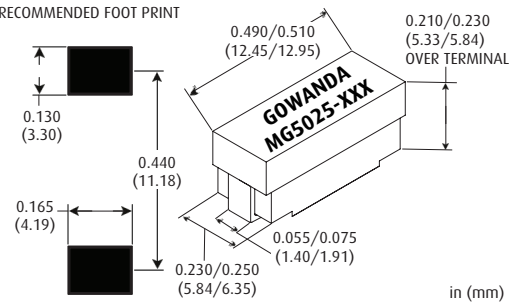
RECOMMENDED FOOT PRINT
