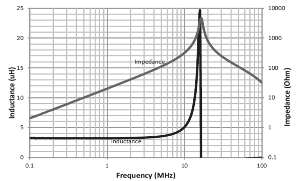
HCM1A1305V3-3R3-R
