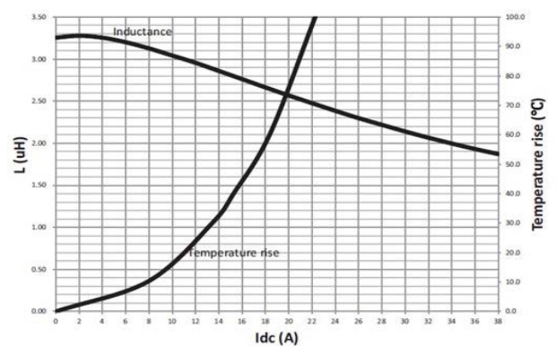
HCM1A1305V3-3R3-R
