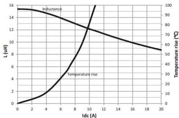
HCM1A1305V3-150-R
