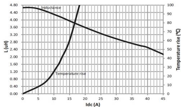
HCM1A1305V3-4R7-R
