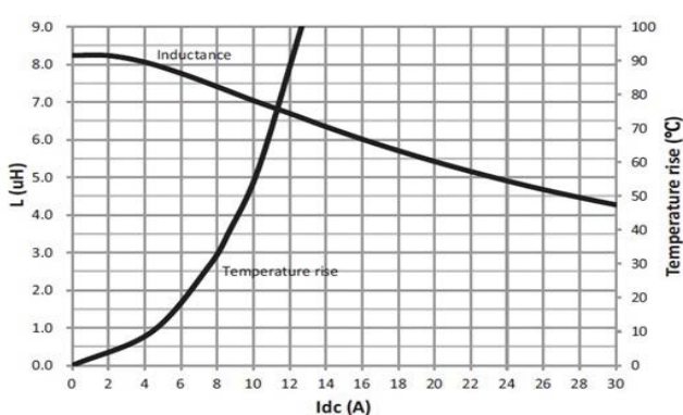
HCM1A1305V3-8R2-R
