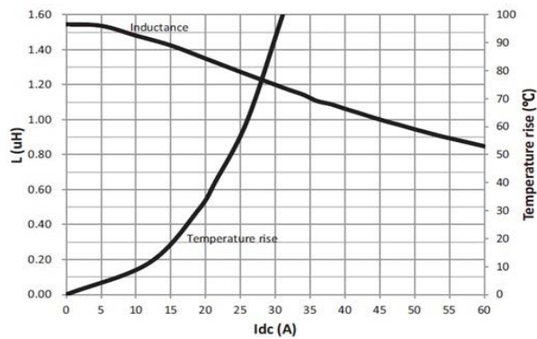
HCM1A1305V3-1R5-R
