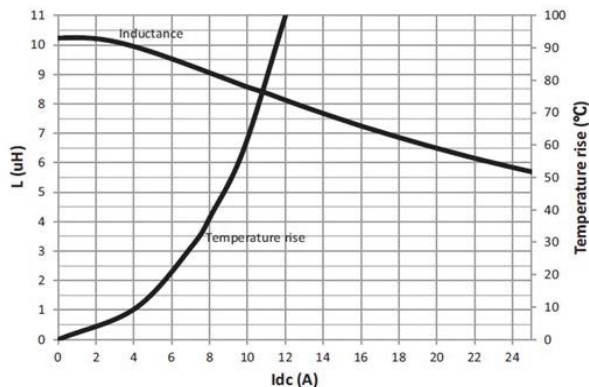
HCM1A1305V3-100-R
