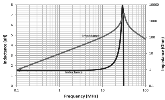
HCM1A1305V3-1R5-R
