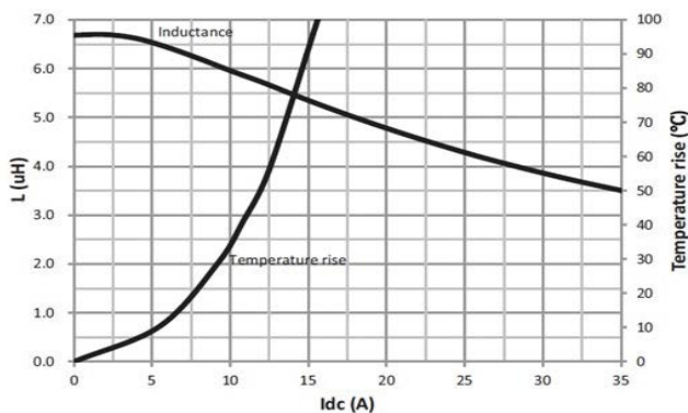
HCM1A1305V3-6R8-R
