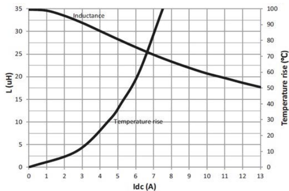
HCM1A1305V3-330-R
