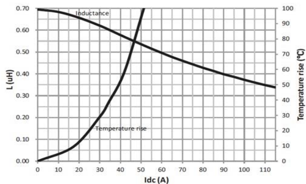
HCM1A1305V3-R68-R
