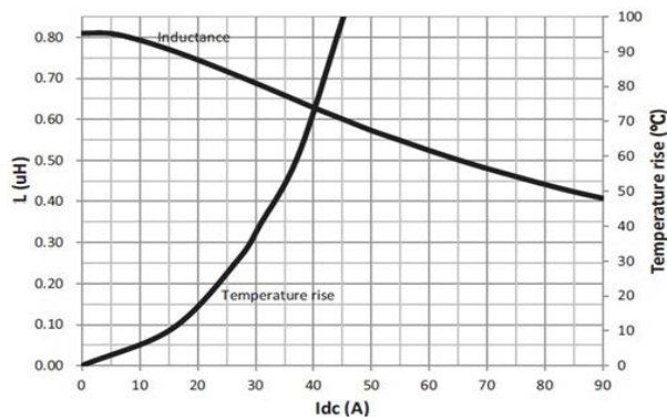
HCM1A1305V3-R82-R
