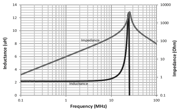
HCM1A1305V3-2R2-R
