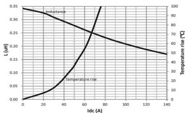
HCM1A1305V3-R33-R
