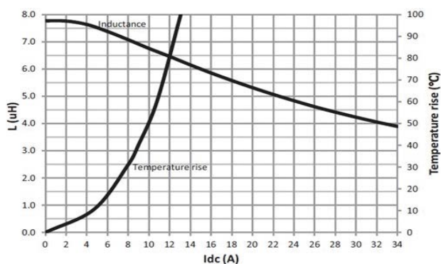
HCM1A1305V3-7R8-R
