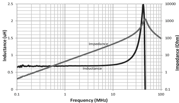
HCM1A1305V3-R68-R
