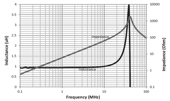
HCM1A1305V3-1R0-R
