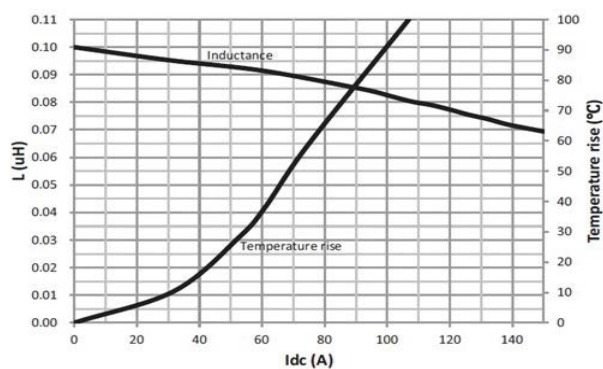
HCM1A1305V3-R10-R
