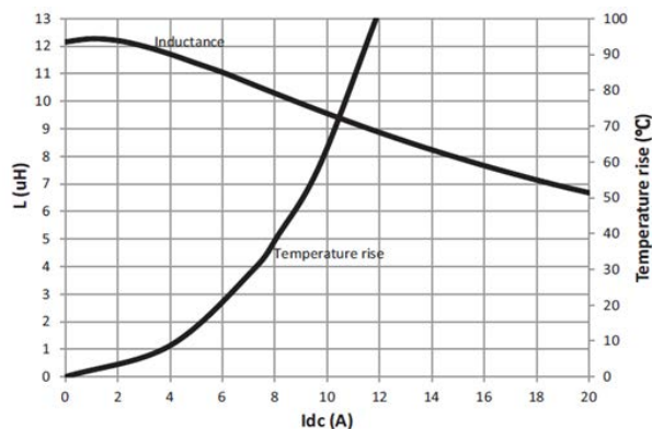
HCM1A1305V3-120-R
