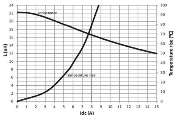
HCM1A1305V3-220-R
