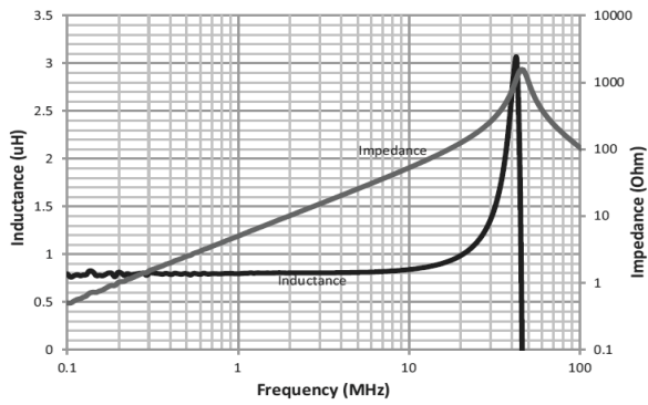
HCM1A1305V3-R82-R
