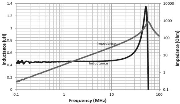
HCM1A1305V3-R47-R
