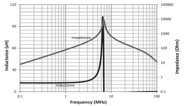
HCM1A1305V3-120-R
