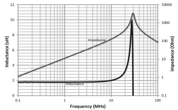
HCM1A1305V3-1R8-R
