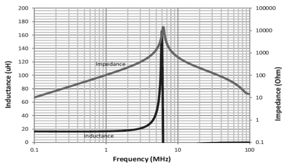
HCM1A1305V3-150-R
