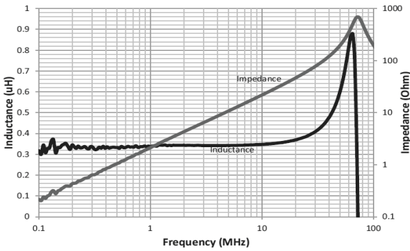
HCM1A1305V3-R33-R
