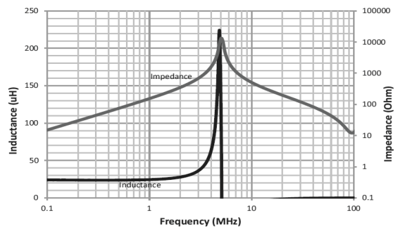
HCM1A1305V3-220-R
