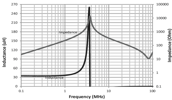
HCM1A1305V3-330-R
