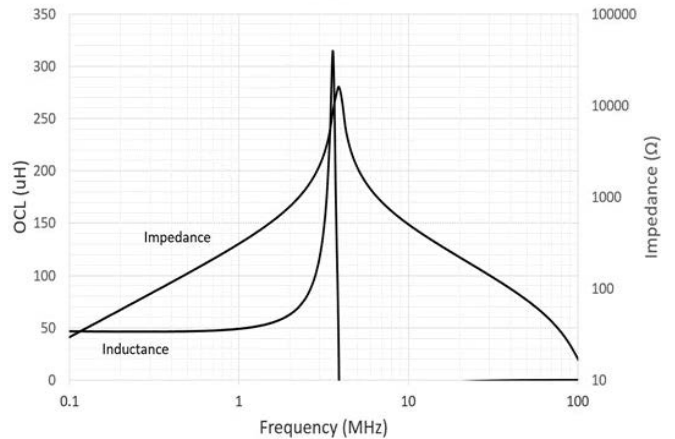
HCM1A1104V3-470-R
