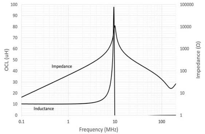
HCM1A1104V3-100-R
