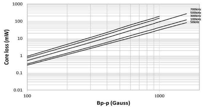
HCM1A1104V3-470-R
