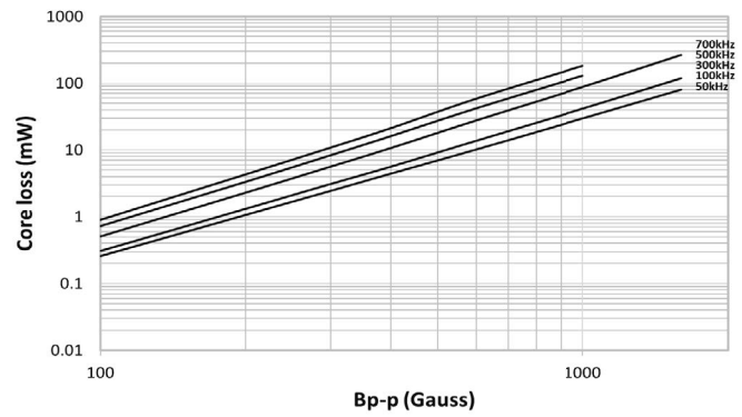
HCM1A1104V3-3R3-R
