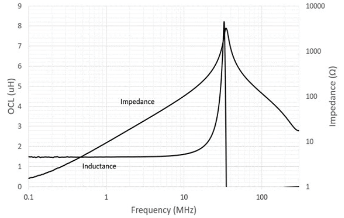
HCM1A1104V3-1R5-R
