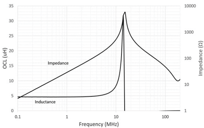
HCM1A1104V3-4R7-R
