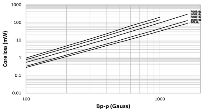
HCM1A1104V3-R56-R
