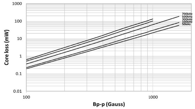
HCM1A1104V3-1R5-R
