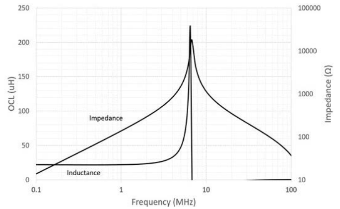
HCM1A1104V3-220-R
