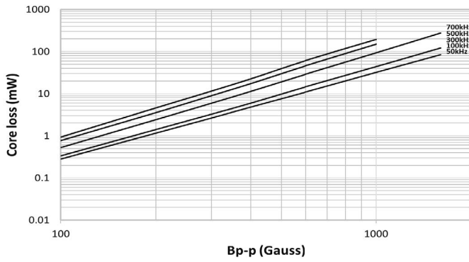
HCM1A1104V3-6R8-R
