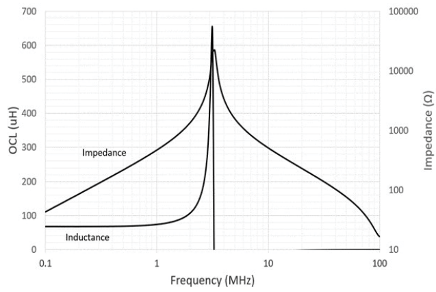
HCM1A1104V3-680-R
