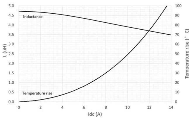
HCM1A1104V3-4R7-R
