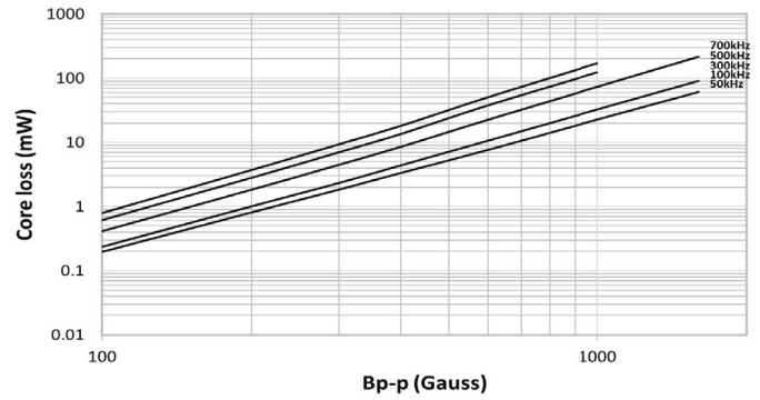
HCM1A1104V3-100-R
