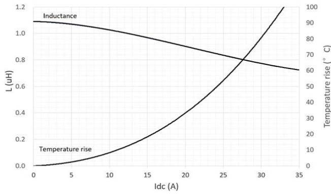
HCM1A1104V3-1R0-R
