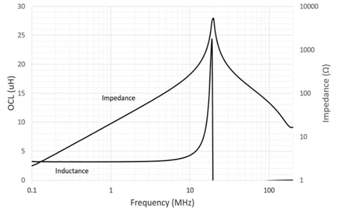
HCM1A1104V3-3R3-R
