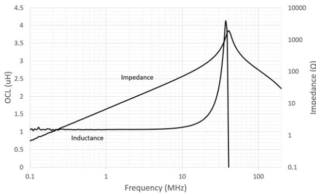
HCM1A1104V3-1R0-R
