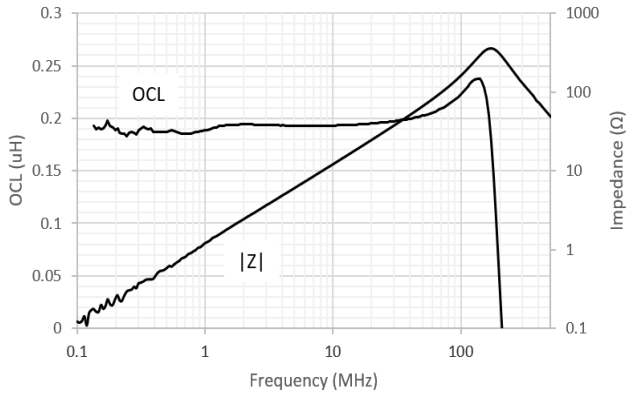
HCM1A0503V3-R20-R
