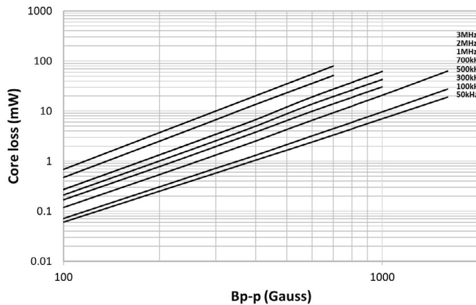
HCM1A0503V3-2R2-R
