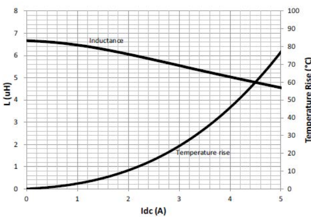
HCM1A0503V3-6R8-R
