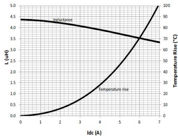
HCM1A0503V3-4R7-R
