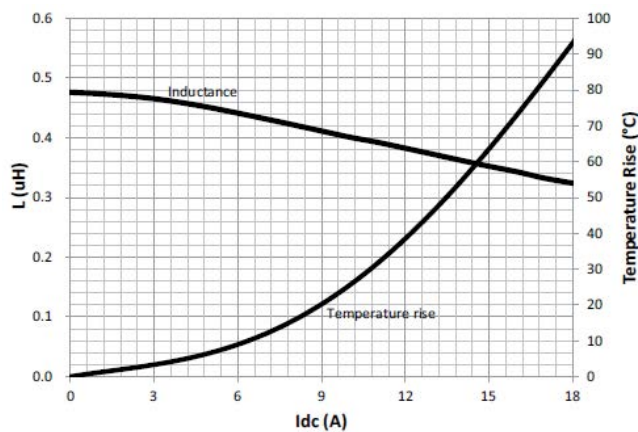
HCM1A0503V3-R47-R
