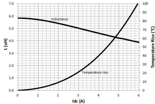
HCM1A0503V3-100-R
