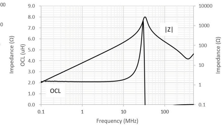
HCM1A0503V3-2R2-R
