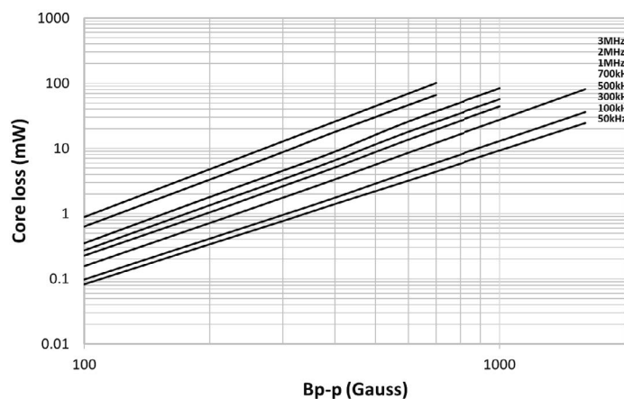
HCM1A0503V3-3R3-R
