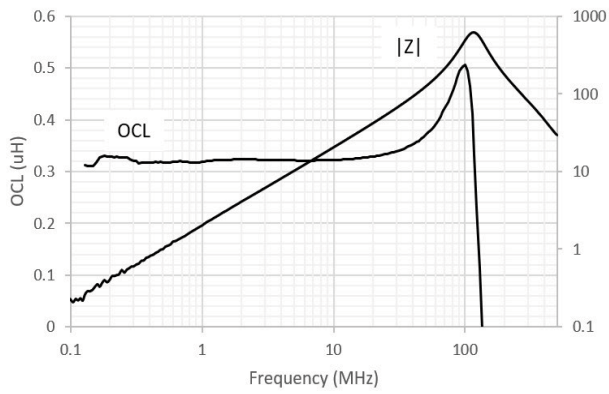
HCM1A0503V3-R33-R
