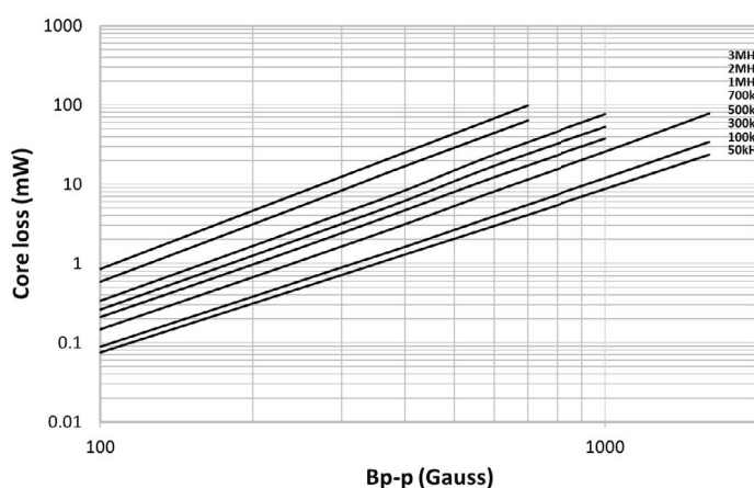
HCM1A0503V3-2R2-R
