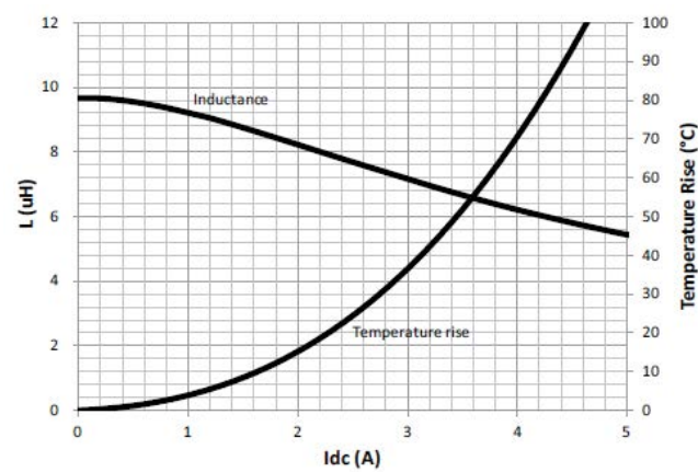
HCM1A0503V3-100-R
