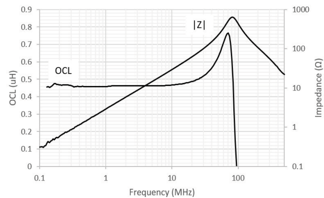
HCM1A0503V3-R47-R
