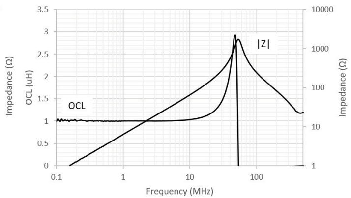
HCM1A0503V3-1R0-R
