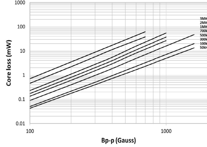
HCM1A0503V3-R33-R
