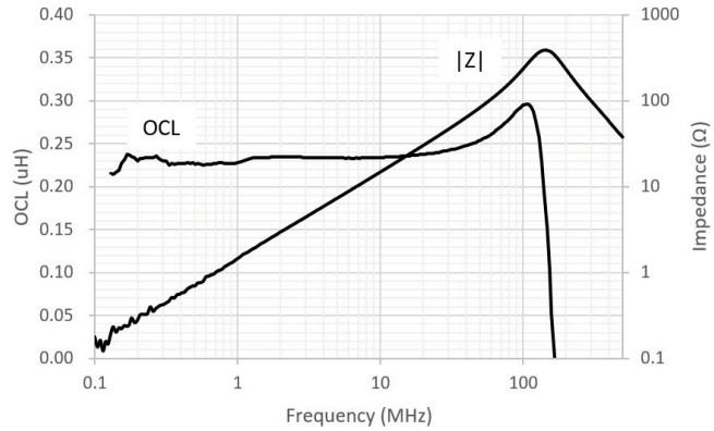
HCM1A0503V3-R22-R
