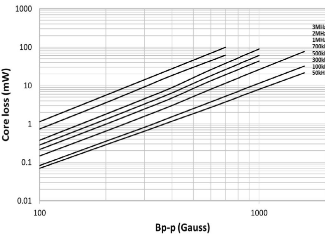
HCM1A0503V3-R35-R
