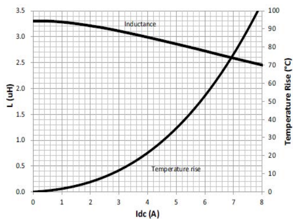
HCM1A0503V3-3R3-R
