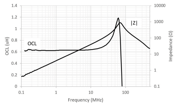
HCM1A0503V3-R68-R
