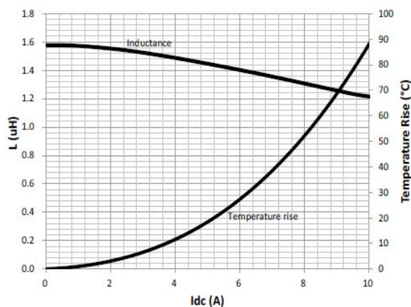
HCM1A0503V3-1R5-R
