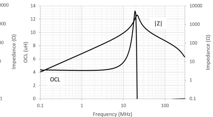
HCM1A0503V3-4R7-R
