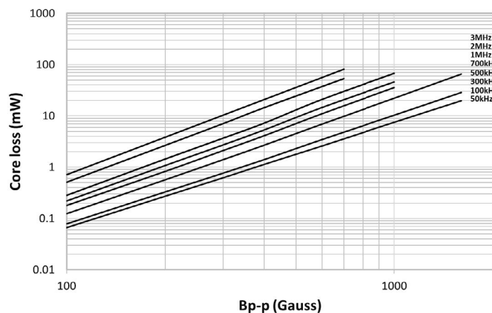
HCM1A0503V3-1R5-R
