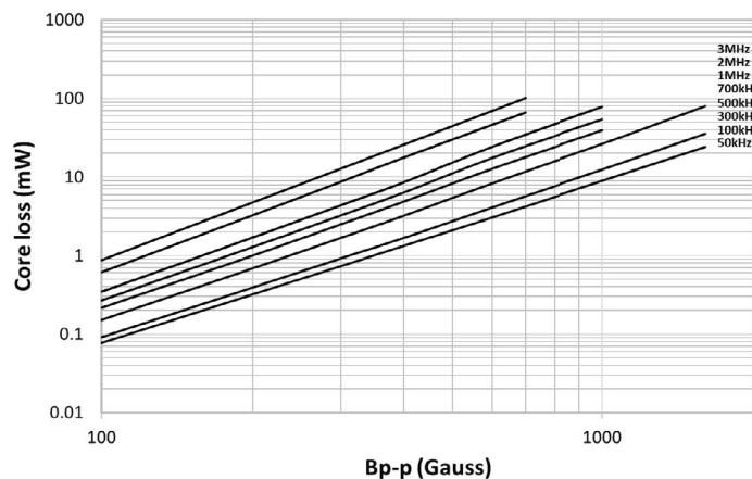
HCM1A0503V3-3R3-R
