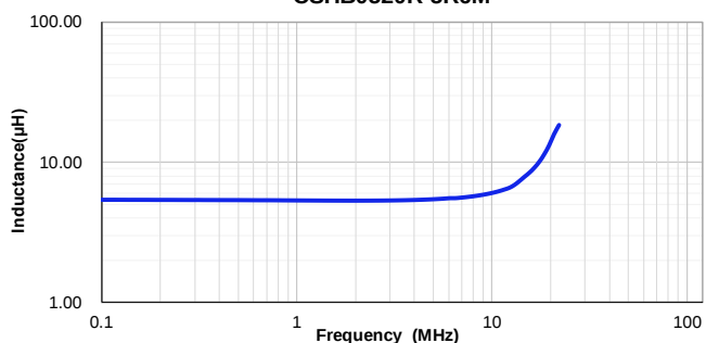
CSHB0520R-5R6M
