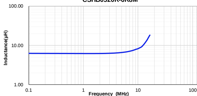
CSHB0520R-6R8M
