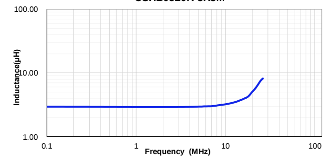
CSHB0520R-3R3M
