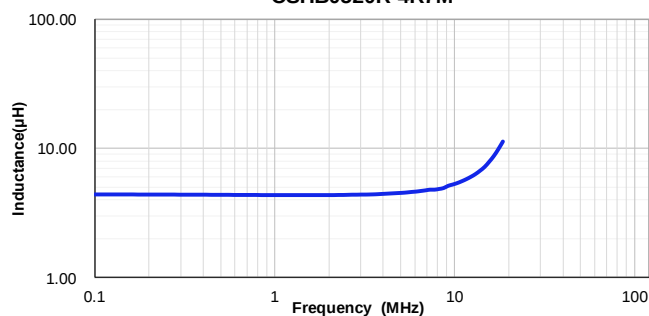
CSHB0520R-4R7M
