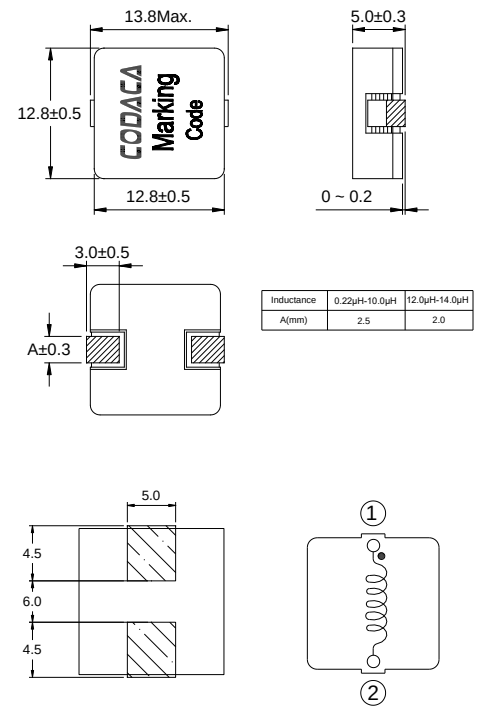
Typical Land Pattern
