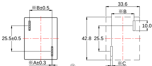
Reference Hole Pattern
