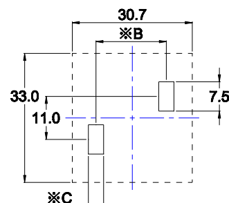
Typical Hole pattern
