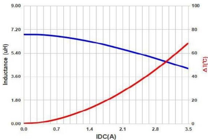
AMELA4012S-6R8M
