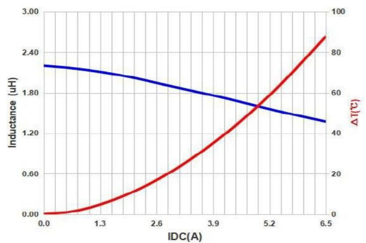
AMELA4012S-2R2M
