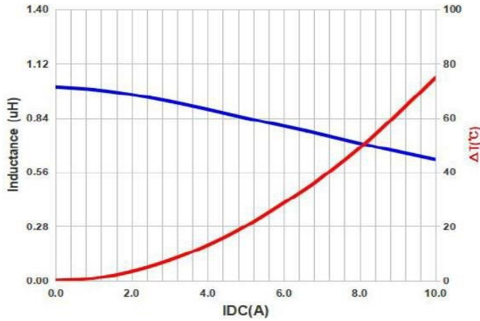
AMELA4012S-1R0M
