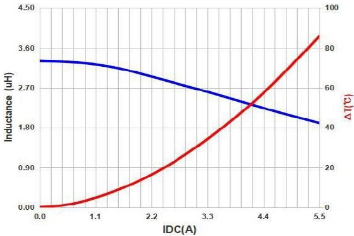
AMELA4012S-3R3M
