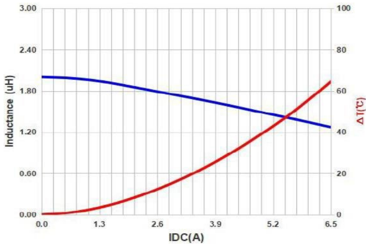
AMELA4012S-2R0M
