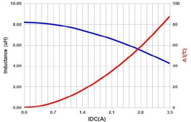
AMELA4012S-8R2M
