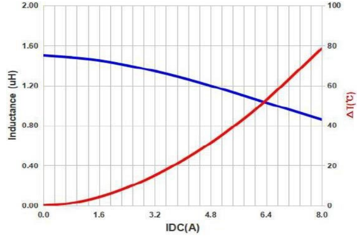
AMELA4012S-1R5M
