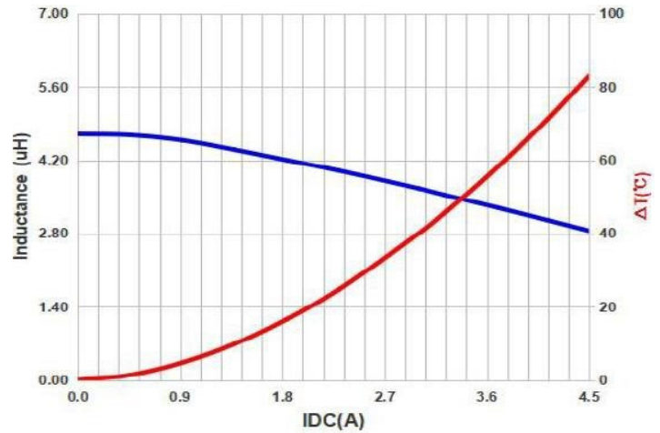
AMELA4012S-4R7M
